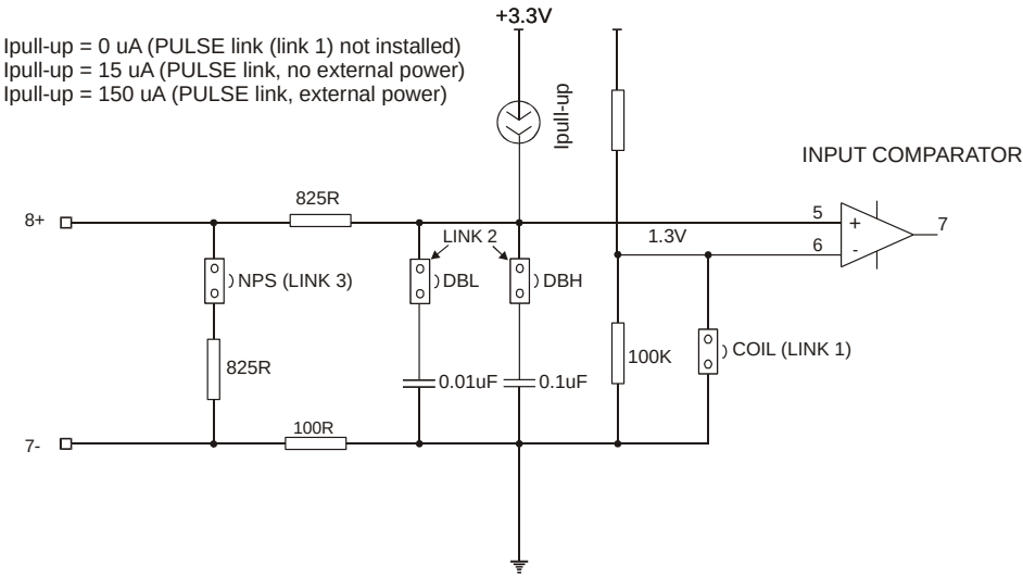
SIMPLIFIED FREQUENCY INPUT CIRCUIT
