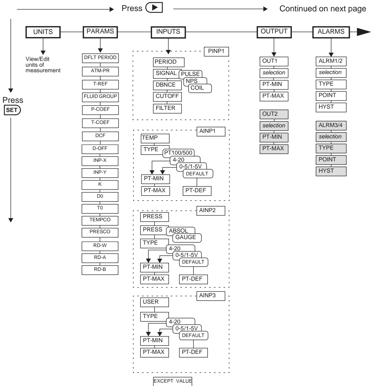
Figure 13 and Figure 14 show the keys for moving around the calibration menu tree in Calibration View or Set mode.
