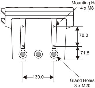
Enclosure with 3 x M20 Gland holes
