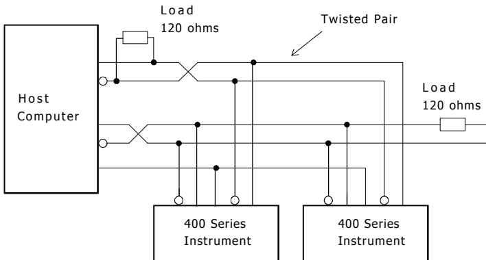
Figure 1 RS422 Interface
