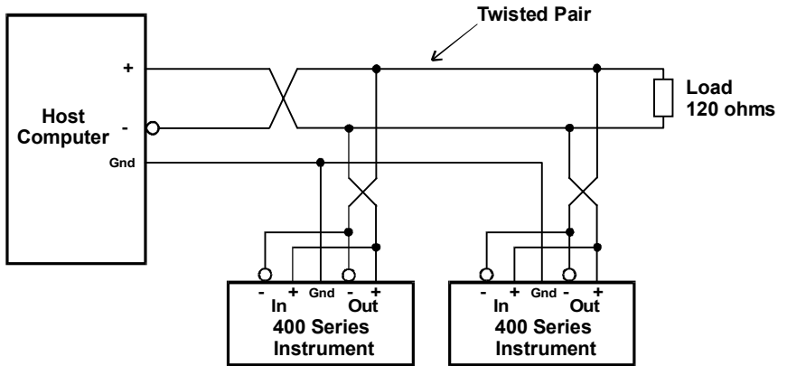
Figure 2 RS485
