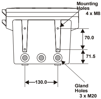
Enclosure with 3 x M20 Gland holes
