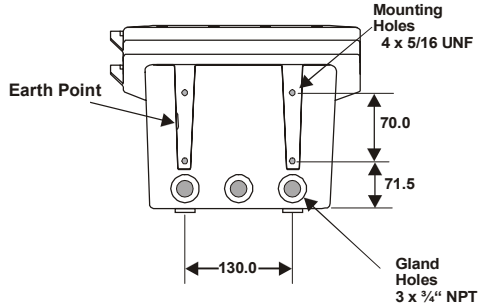
Enclosure with 3 x 3/4" NPT Gland holes
