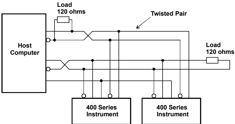
Figure 1 RS422 Interface
